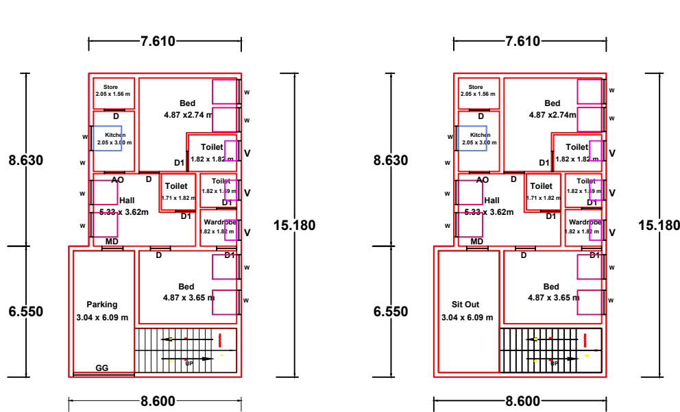
GROUND FLOOR (East Facing)
