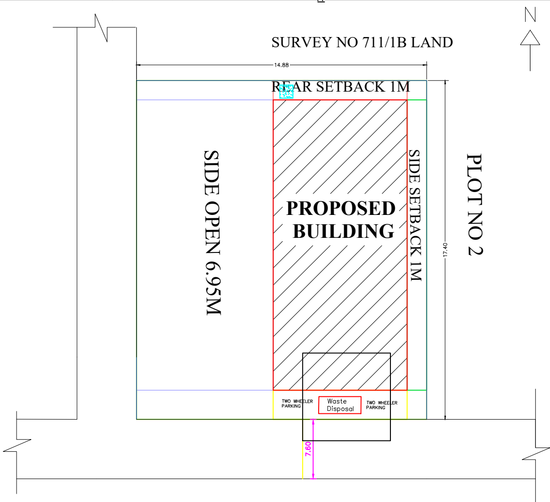
SITE PLAN
