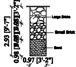
SECTION OF RAIN WATER COLLECTION PITS - ONTS
