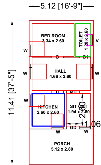
GROUND FLOOR PLAN (EAST FACING)
