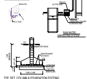
TYP. DET. COLUMN & FOUNDATION FOOTING
