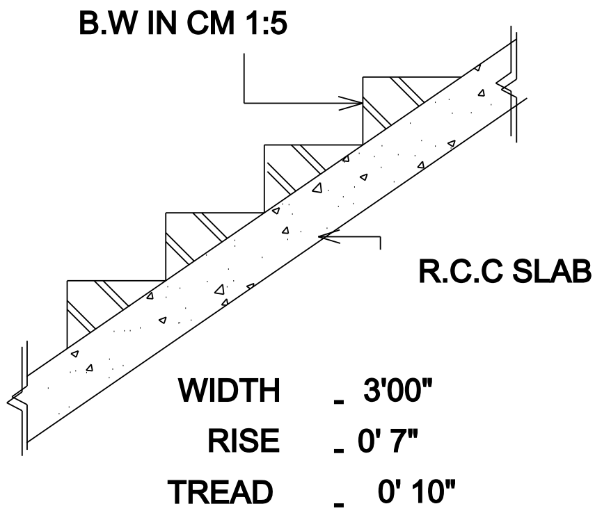
STAIR DETAILS NOT TO SCALE
