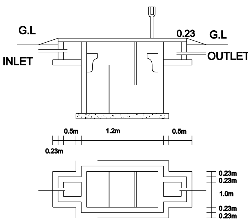
SEPTIC TANK DETAILS NOT TO SCALE
