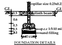
FOUNDATION DETAILS
