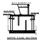
SEPTIC TANK SECTION
