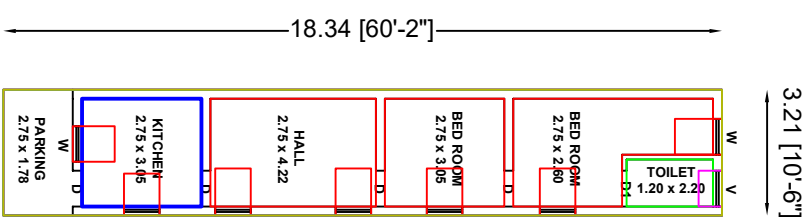
GROUND FLOOR PLAN (EAST FACING)
