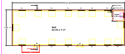
Proposed Ground Floor Plan (West Facing)
