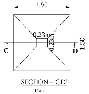
SECTION - 'CD' Plan
