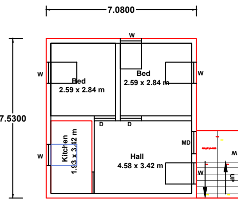
EXISTING GROUND FLOOR
