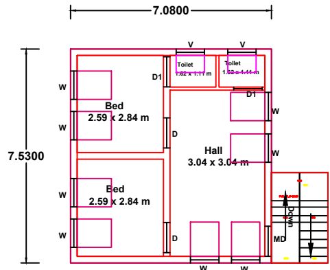
PROPOSED FIRST FLOOR
