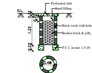
PERCOLATION PIT
