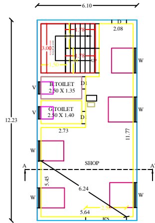
GROUND FLOOR PLAN (SOUTH FACING)
