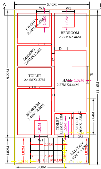
PRO. FIRST FLOOR PLAN
