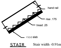
STAIR Stair width -0.91m
