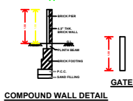
COMPOUND WALL DETAIL
