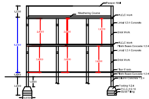
Section Section - AA
