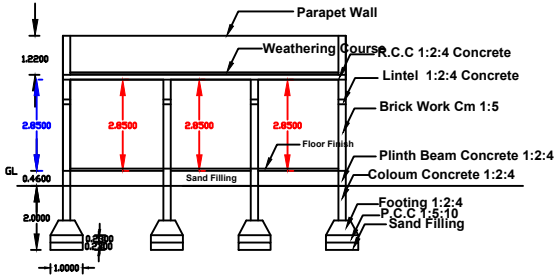
Section Section - AA
