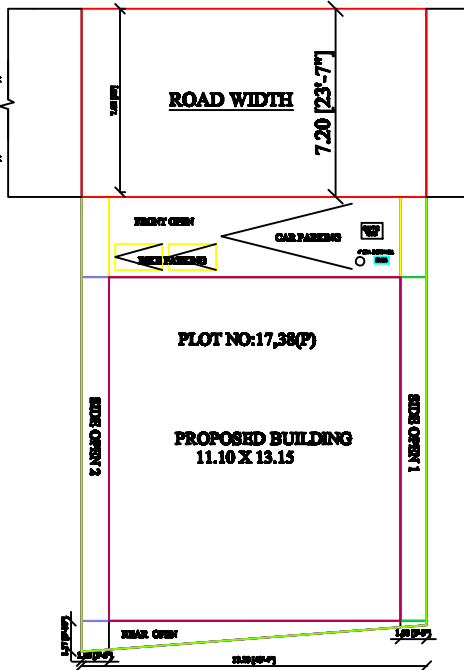
SITE PLAN
