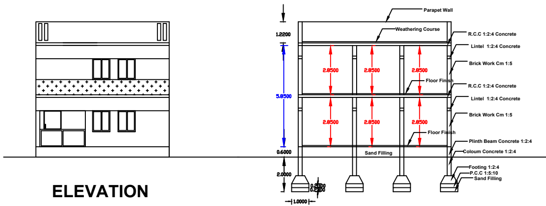
Section Section - AA
