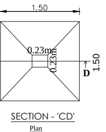
SECTION - 'CD' Plan
