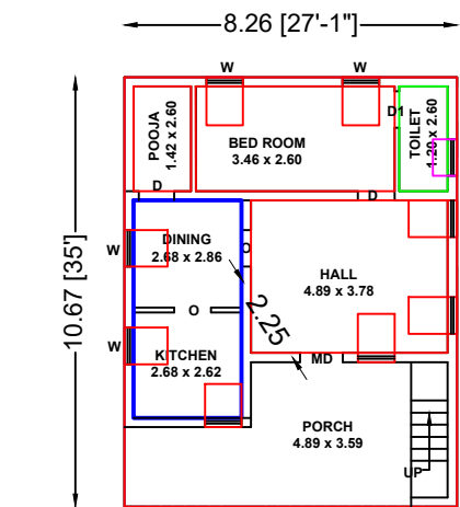
GROUND FLOOR PLAN (EAST FACING)
