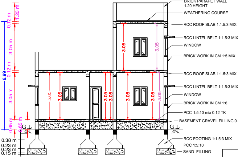
SECTION S-S
