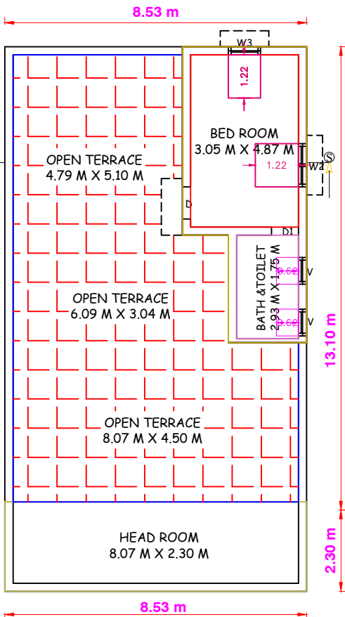
FIRST FLOOR PLAN [NORTH FACING]
