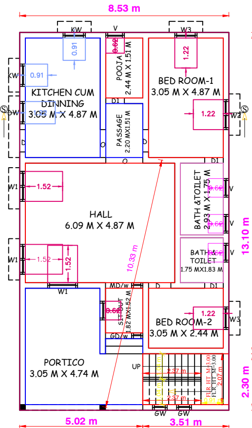
GROUND FLOOR PLAN [NORTH FACING]
