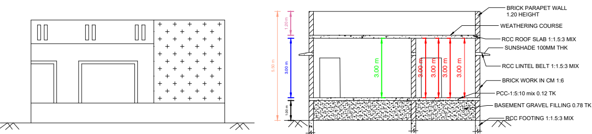
FRONT ELEVATION
