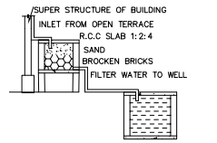
RAINWATER HARVESTING
