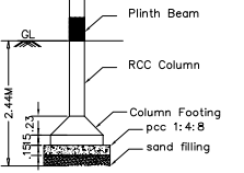
Column Footing
