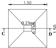
SECTION - 'CD' Plan
