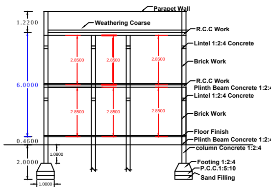
SECTION SECTION - AB
