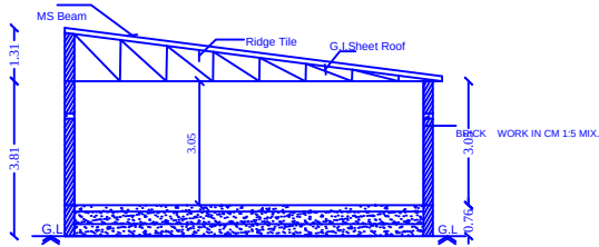
Section on-"AA"
