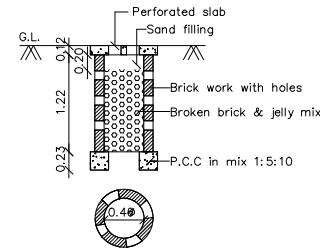
PERCOLATION PIT FOR 30Sq.m. (Scale:- 1:50)
