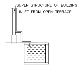
RAINWATER HARVESTING
