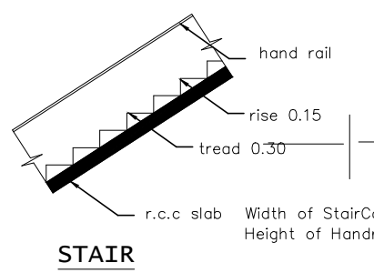
STAIR
