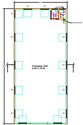
Proposed Ground Floor Plan
