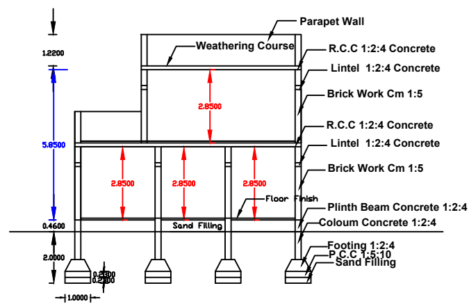
Section Section - AA
