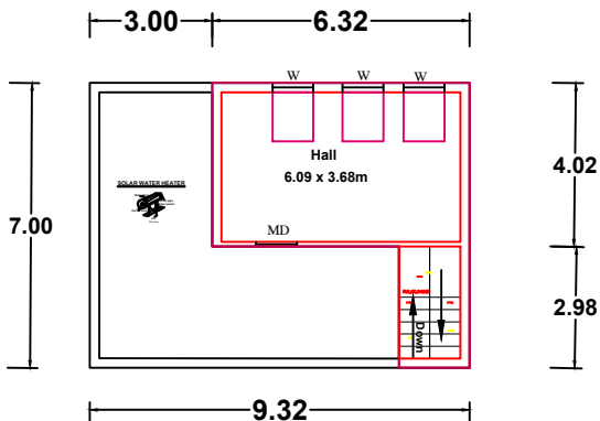
FIRST FLOOR PLAN & OPEN TERRACE
