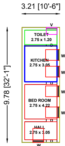
GROUND FLOOR PLAN (EAST FACING)
