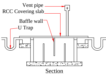
Section
