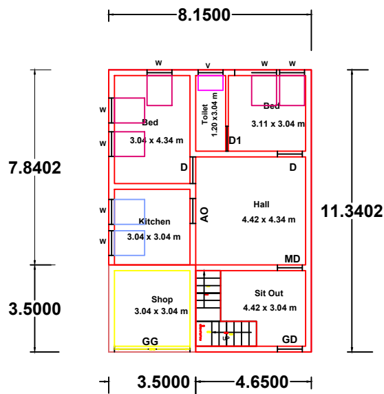
GROUND FLOOR PLAN ( EAST FACING )
