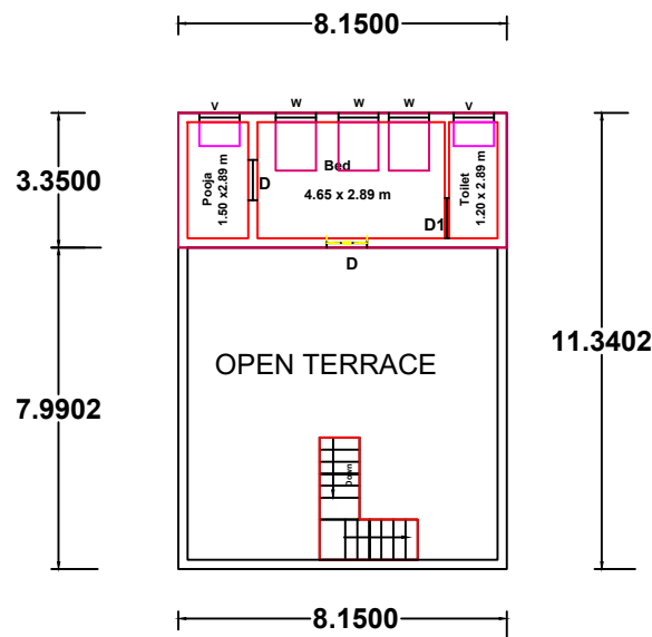
FIRST FLOOR PLAN ( EAST FACING )
