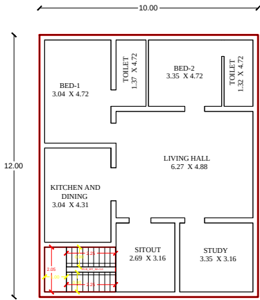
EXISTING GROUND FLOOR PLAN
