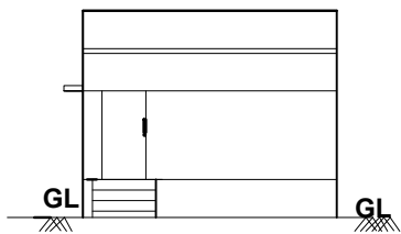
FRONT ELEVATION
