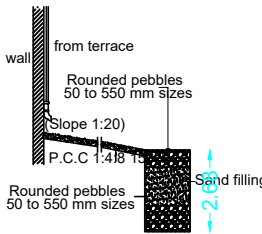
PLAN OF RAIN WATER HARVESTING
