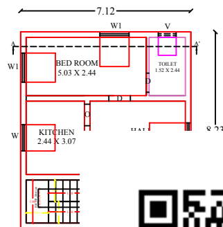
GROUND FLOOR PLAN (EAS)
