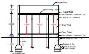
SECTION SECTION - AB
