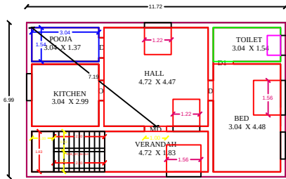
GROUND FLOOR PLAN EAST FACING
