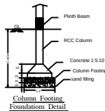
Column Footing
