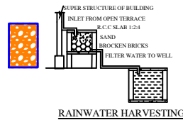
RAINWATER HARVESTING
