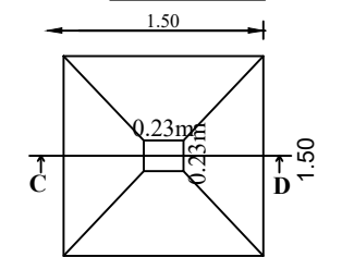
SECTION - 'CD'
