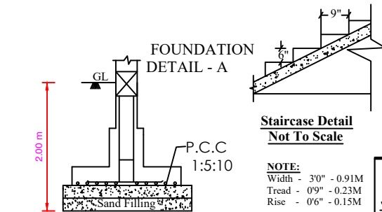
Isolated Footing -A (1.50X1.50) (Not to Scale)
