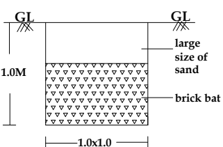
RAINWATER HARVESTING
