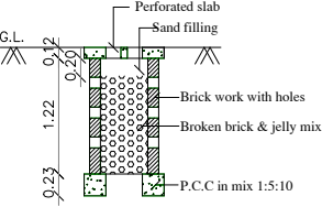
PERCOLATION PIT
