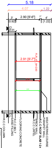
SECTION ON AA
