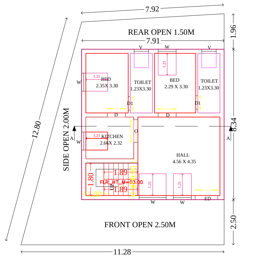
GROUND FLOOR (EAST FACING)
