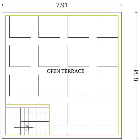
OPEN TERRACE
