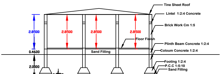
Section Section - AA
