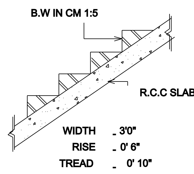
STAIR DETAILS
