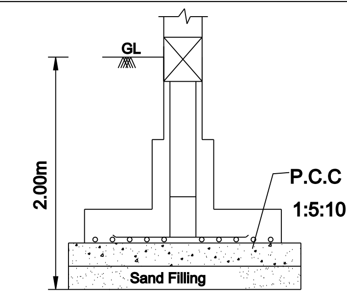
FOUNDATION DETAIL
