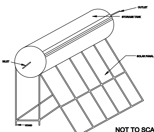
SOLAR WATER HEATER DETAILS
