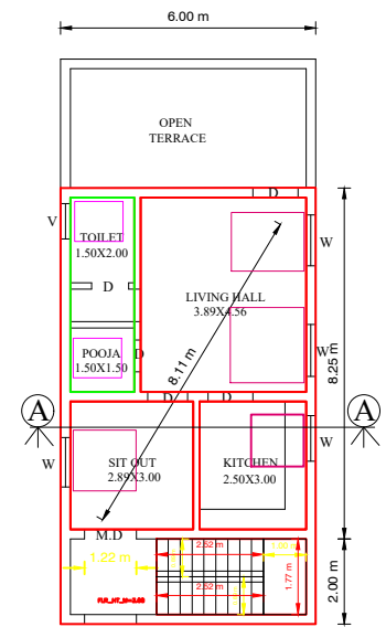
FOOR PLAN
