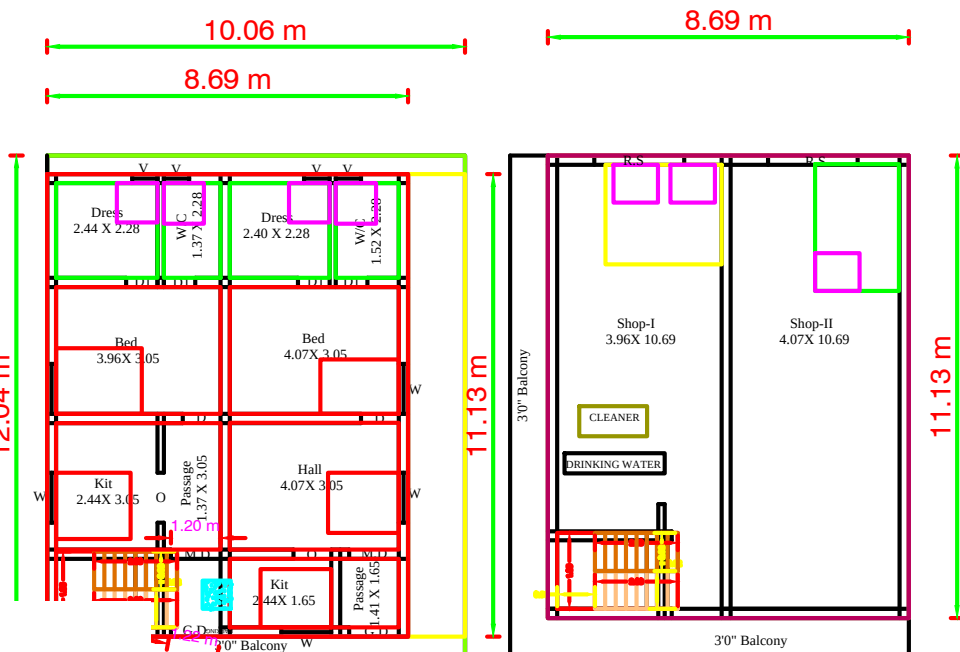
FIRST FLOOR PLAN(West-Facing)
