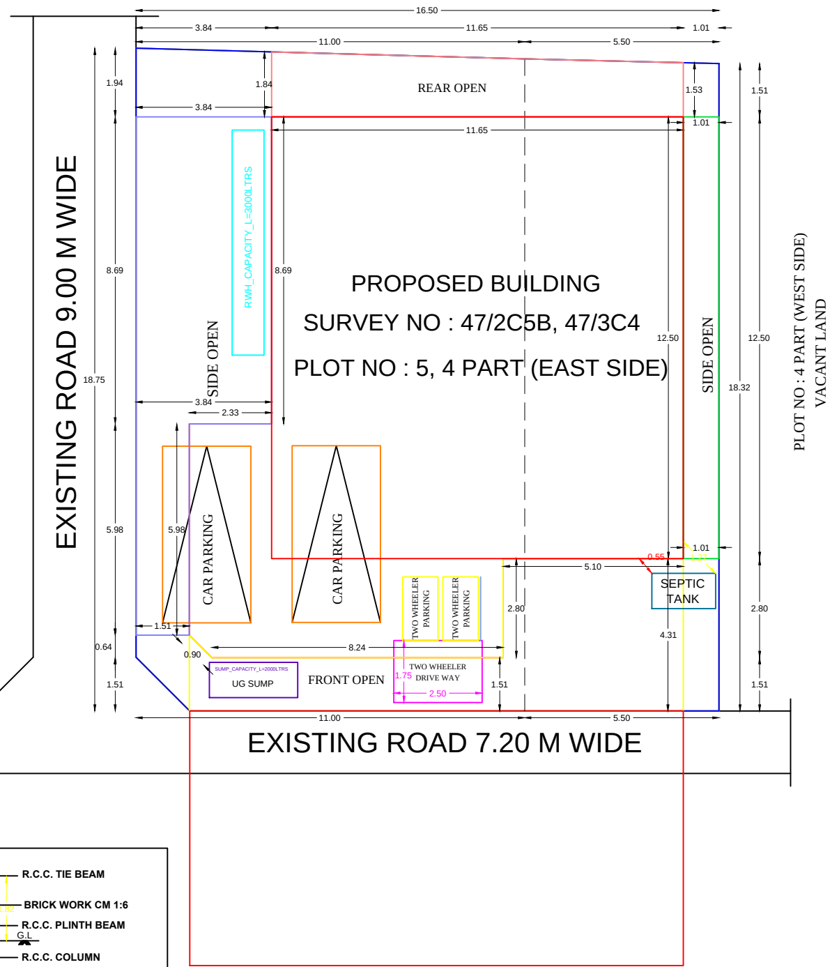
SITE PLAN
