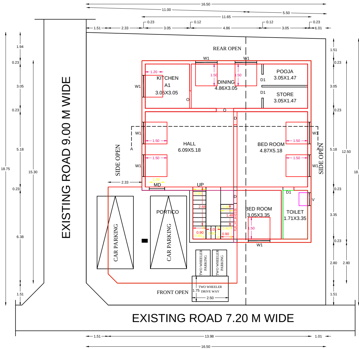
GROUND FLOOR PLAN (ORTH FACING)
