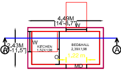
GROUND FLOOR PLAN SCALE - 1 : 100
