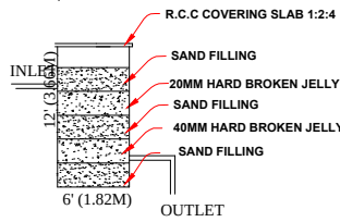
Waste Water Recycle Unit Not To Scale
