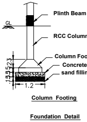
Column Footing
